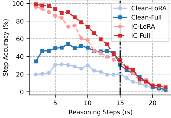
Figure 5: Step accuracy of models trained with Clean or IC data using LoRA or continued pretraining.
