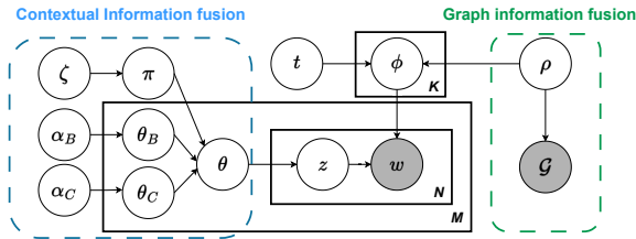
Figure 1: The document generation process of CGTM, where N is the number of words in M documents.
