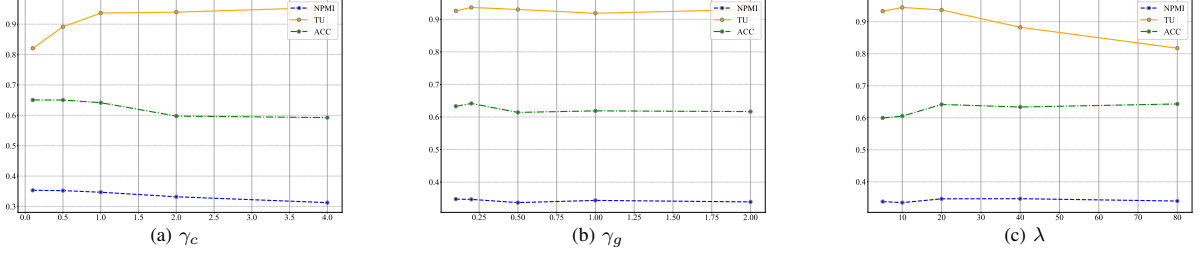
Figure 6: Performances under different values of hyper-parameters on 20News.
