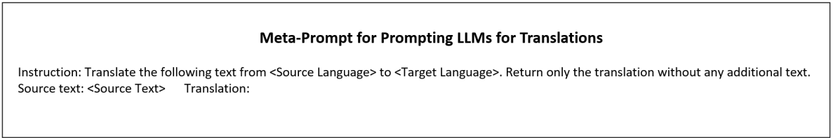
Figure 6: The prompt template used for prompting LLMs for translations.
