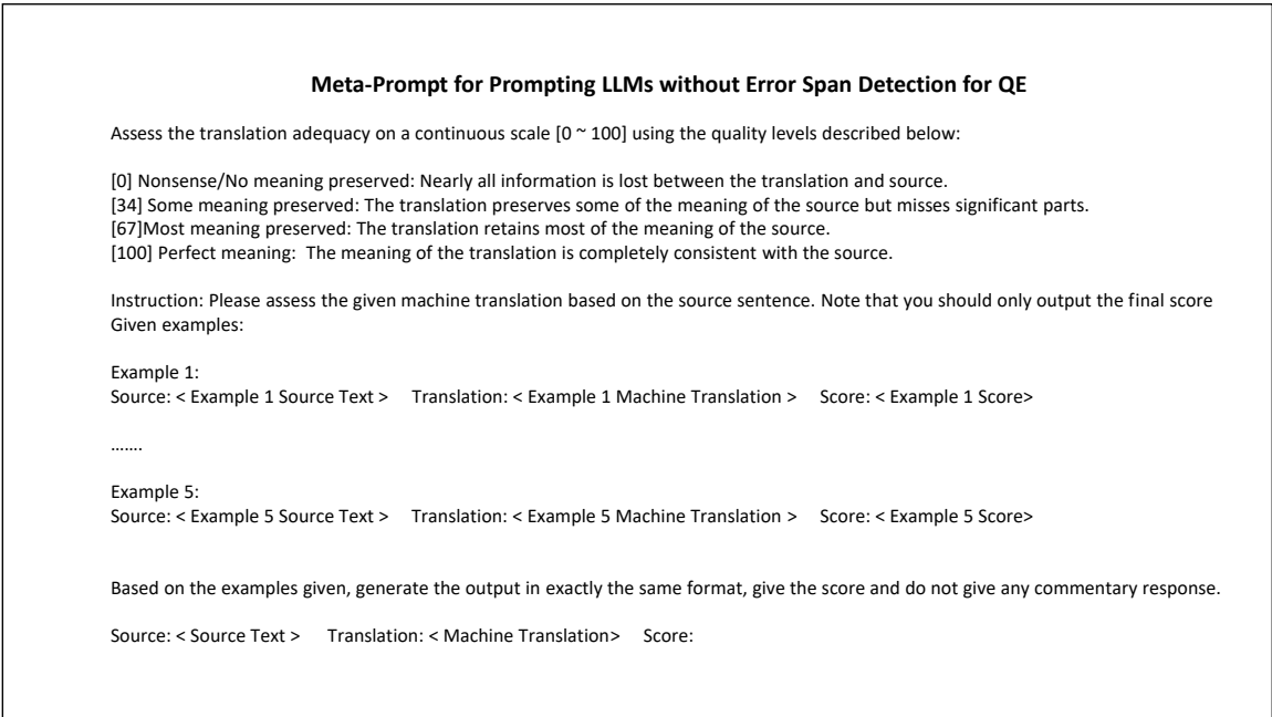
Figure 9: The prompt template used for prompting LLMs without error span detection for QE.
