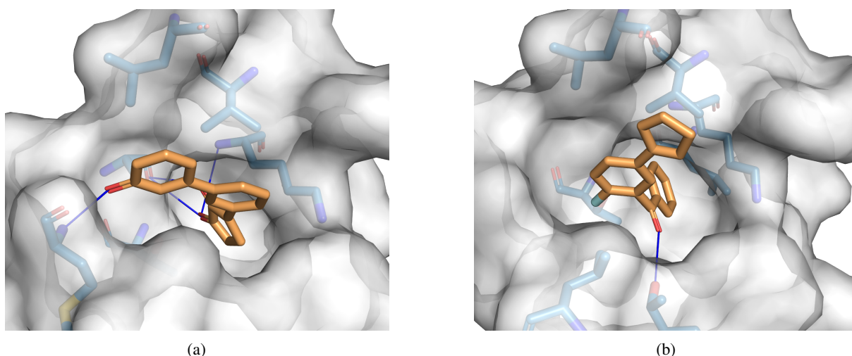
Figure A3: (a) Docking of NL-2 to EGFR pocket, with hydrogen bonds shown as solid blue lines. (b) Docking of NL-3 to EGFR pocket, with hydrophobic van der Waals contacts shown using solid blue lines.
