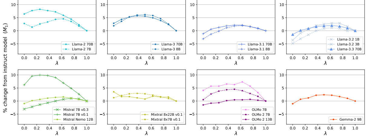
Figure 1: Performance on the in-context learning benchmark: fractional difference (percent value) between the performance of each partially adapted model M_\lambda and the instruct baseline M_1 for all the models we have tested.
