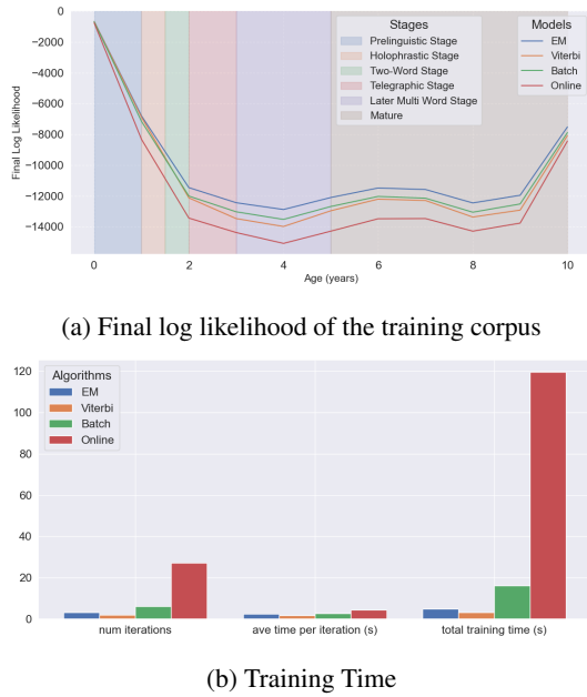
Figure 6: Training statistics of different EM algorithms.
