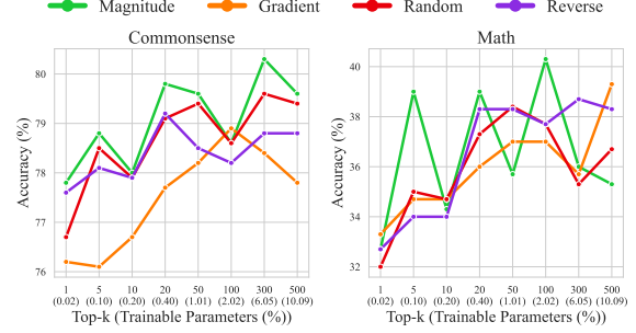
Figure 7: Comparison of different parameter selection strategies for involving neurons for the fine-tuning process. Among all input connections for each neuron in the network, Top- k connection with highest magnitude ( Magnitude ), highest gradient absolute value ( Gradient ), lowest magnitude ( Reverse ) are selected for training using addition-based method. Random means randomly selecting Top- k input connections per neuron.
