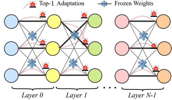
Figure 1: Overview of NeuroAda. For each neuron, top-1 weights are adapted, while the rest remain frozen. Bold dark indicates selected pretrained weights; red dashed edges represent newly introduced trainable parameters.
