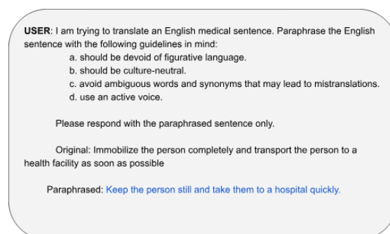
Figure 5: Example prompt and model completion (in text color blue) for paraphrasing.
