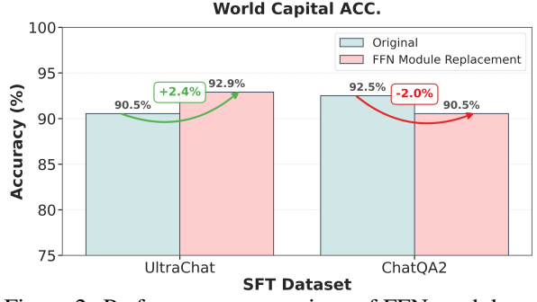
Figure 2: Performance comparison of FFN module replacement. Accuracy is measured on the World Capital.
