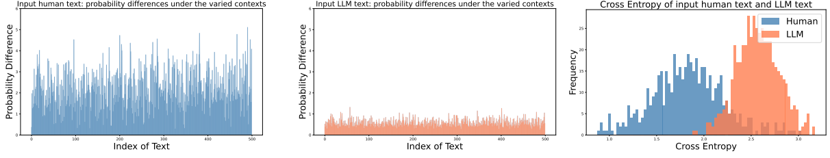
(a) Prob. differences of human texts. (b) Prob. differences of LLM texts. (c) Cross entropy of input texts.
