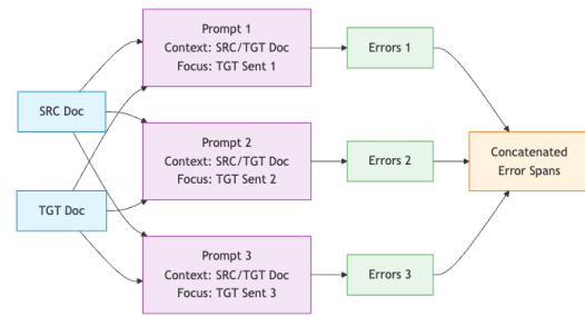
Figure 3: FSP on a three-sentence document.
