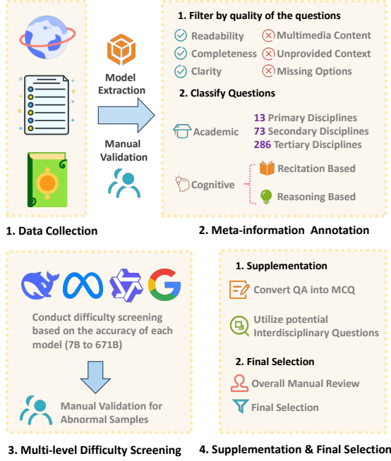
Figure 2: An overview of NOVA-63’s data processing pipeline.
