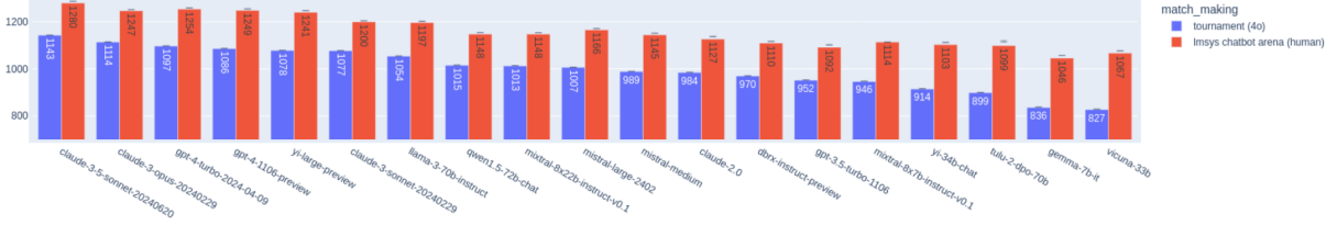
Figure 8: BT preference of the model with gpt-4o judge on the full set of Arena-Hard-Auto (Li et al., 2024) prompts. Arena-Lite result (bootstrapped median over 1000 samples of 500 trials) is in blue, plotted alongside the ratings from the ground truth leaderboard in red (Chatbot Arena, Hard prompts category ). Error bars are 95% confidence intervals.
