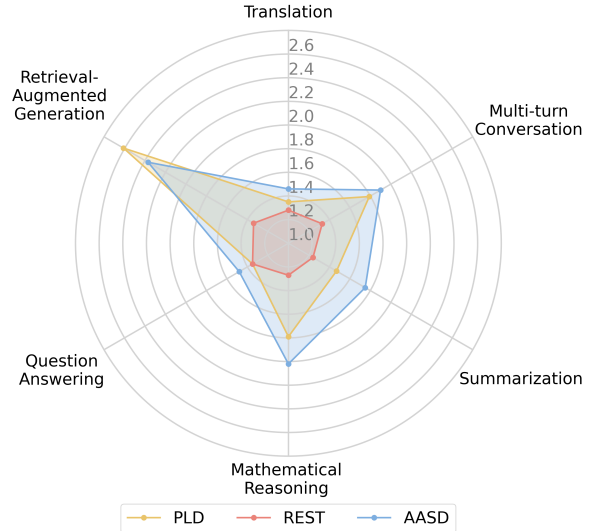
Figure 3: Speed-up ratio on the six different task categories in SpecBench. The center point (1.0x) represents the baseline of autoregressive decoding.
