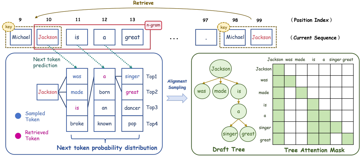
Figure 2: Illustration of alignment sampling. “Jackson is a great” is an n-gram retrieved by the key “Michael Jackson”. According to the output distribution obtained in the prefilling stage, “is” is the token with the third highest probability. The top-1 token “was” and top-2 token “made” are more likely to be generated after “Michael Jackson”. Therefore, we sample two more tokens (“was” and “made” for the 100th position). Token “a” is well aligned with the model output, so we keep it unchanged for the 101st position.
