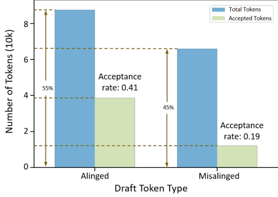
Figure 1: Acceptance rate of aligned and misaligned draft tokens in prompt-based speculative decoding.
