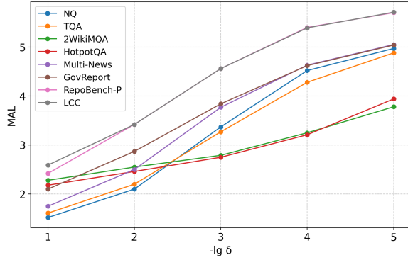
Figure 4: Mean acceptance length of different tasks under threshold verification.
