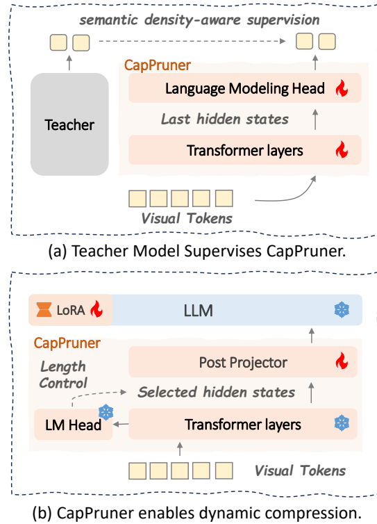
Figure 3: Illustration of the dynamic compression mechanism in CapPruner. (a) Captions generated by a teacher model (a strong captioner) are used to supervise the training of CapPruner, facilitating it to allocate tokens according to scene richness. (b) By leveraging the hidden states of predicted captions as compact representation, CapPruner dynamically adjusts the compression ratio according to the timing of the “end-of-sentence” token prediction.
