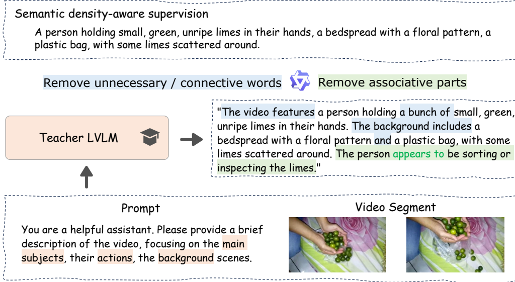
Figure A2: The complete process of obtaining semantic density-aware supervision includes using a powerful LVL as teacher to generate segment descriptions and a subsequent post-processing procedure.
