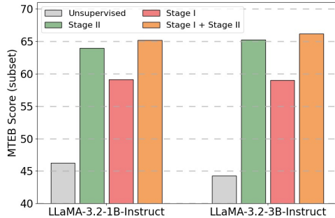
Figure 3: Impact of the two training stages on performance.
