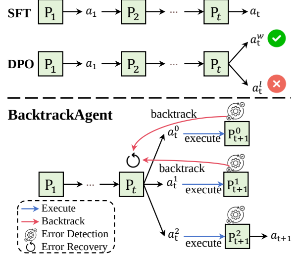
Figure 1: Previous works often struggle to recover from errors, whereas BacktrackAgent utilizes a backtracking mechanism to recover from erroneous pages.
