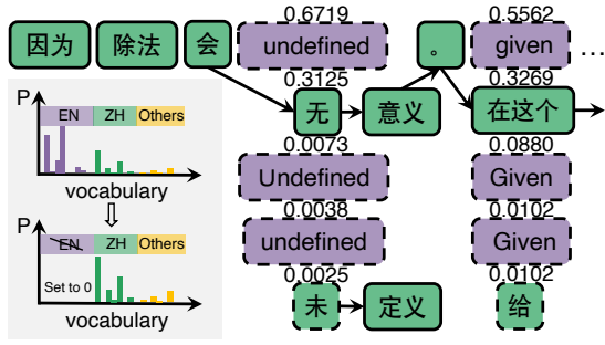
Figure 5: Token-level constrained decoding: We mask out tokens from the undesired language, forcing generation in the target language.
