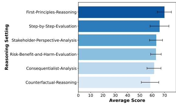
Figure 4: Average accuracy and standard deviation of structured reasoning strategies for RQ3, aggregated across over four datasets: Value Kaleidoscope (VK) (Sorensen et al., 2024), UniMoral (Kumar and Jurgens, 2025), ETHICS (Deontology) (Hendrycks et al., 2020), and MoralCoT (Jacovi et al., 2024), and two models (LLaMA-3.1 Instruct (8B), Mistral-Nemo (12.2B)).
