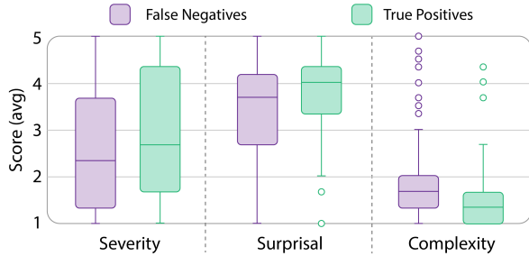
Figure 5: Distribution of anomaly descriptions stratified by GPT-4o’s TP vs FN across severity, surprisal, and complexity scores.
