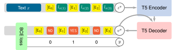
Figure 1: Modeling MLTC as text-to-text with T5. Notations: labels ( l_{\cdot} ), sentinel tokens ( [E_{\cdot}] ).
