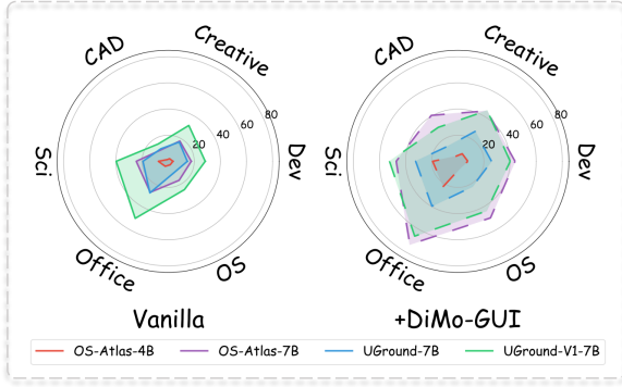
Figure 2: Grounding Performance of DiMo-GUI. By integrating DiMo-GUI, existing models can achieve significant performance improvements on the dataset.
