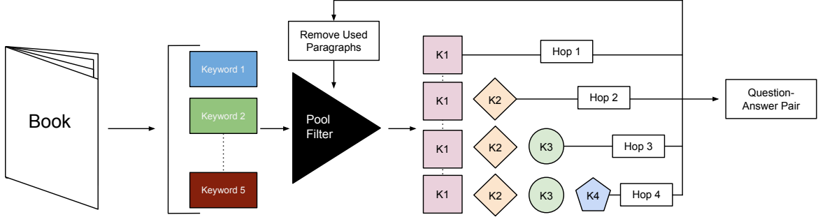
Figure 1: Keyword-guided paragraph-chaining pipeline used to build NOVELHOPQA . See Appendix G for a full example showing multi-hop evolution across four refinement stages.
