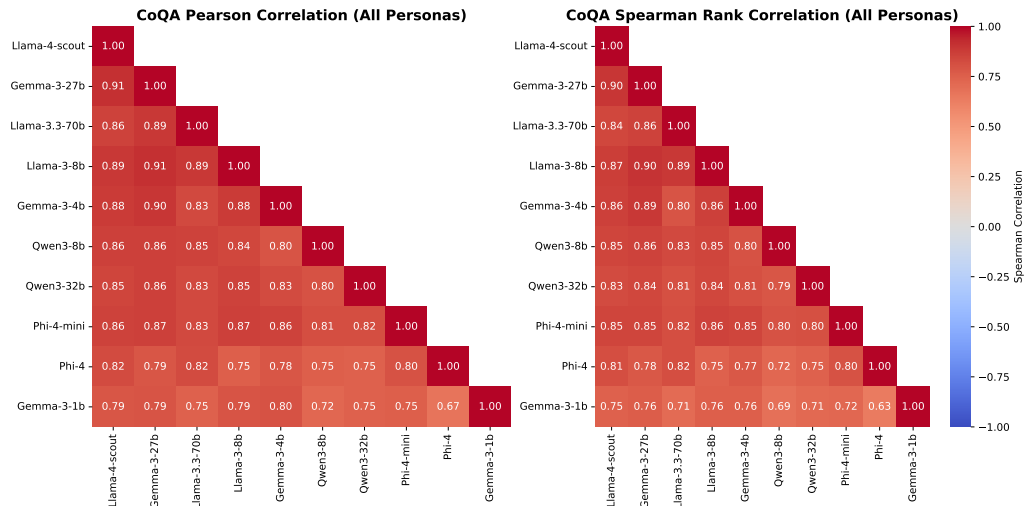
Figure 11: Pearson correlation between all models' performance on CoQA over 1200 personas ( r = 0.84 )
