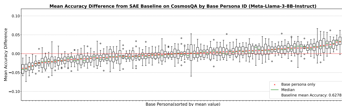
Figure 4: Mean difference in accuracy between each base persona, with the performance varied by the 12 personas with added sociodemographic attributes. The base persona with no sociodemographic attributes is indicated by the red “x.” There is often more variation from adding sociodemographic attributes than from different base personas. This figure is specific to Llama-3-8b on the CosmosQA benchmark, however this pattern holds for all models.
