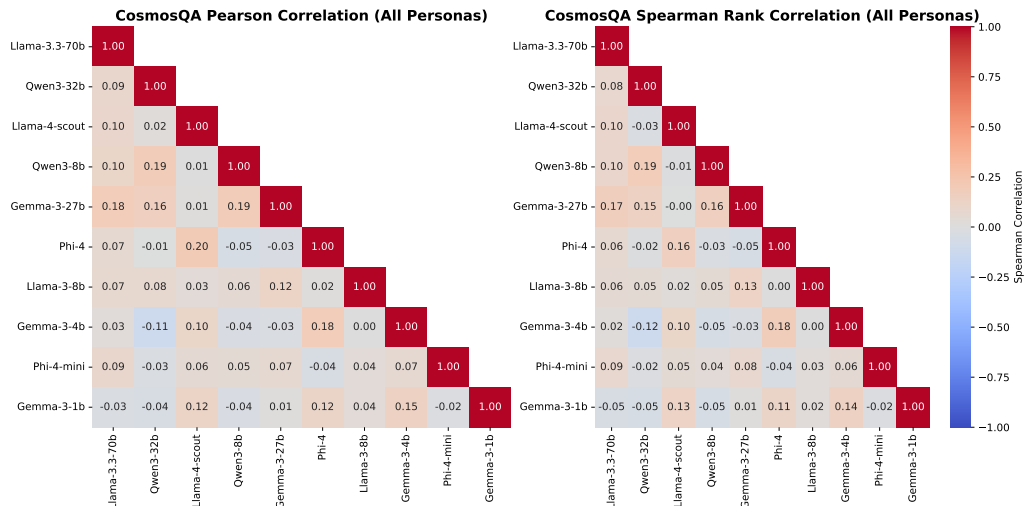
Figure 12: Pearson correlation between all models' performance on CoQA over 1200 personas ( r = 0.07 )
