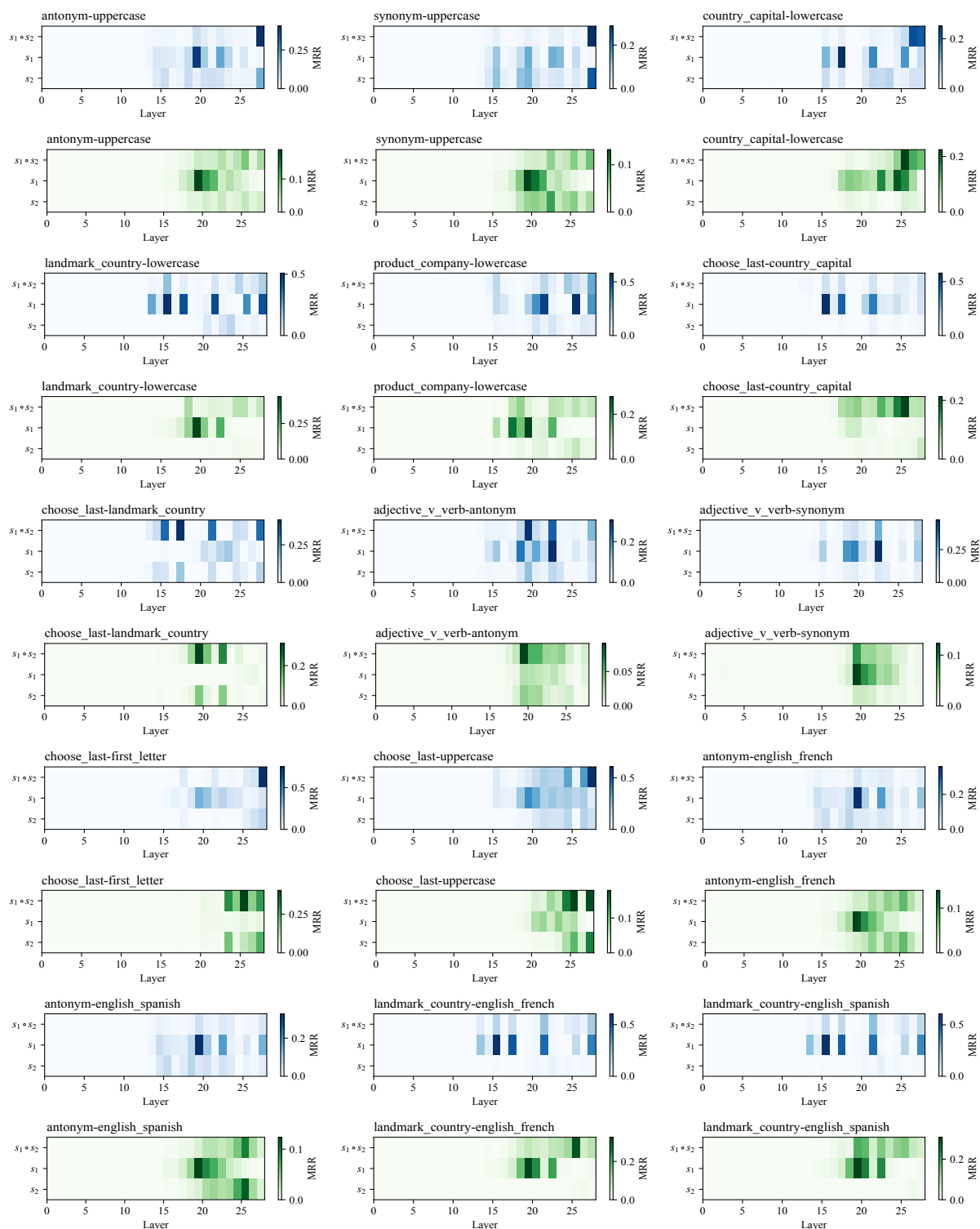
Figure 16: Heatmaps of attention and MLP block decoding results for all tasks in Llama-3.2-3B.
