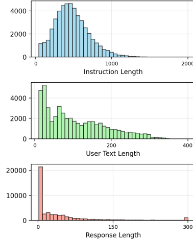
Figure 8: Length distribution in the distillation dataset.
