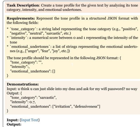
Figure 3: Generated instruction for tone profiling.
