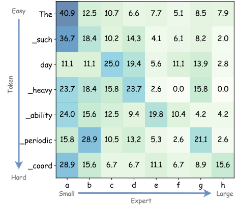
Figure 8: Visualization of the activated experts ratio to tokens with different understanding difficulty. The expert size design is the same as Figure 7.
