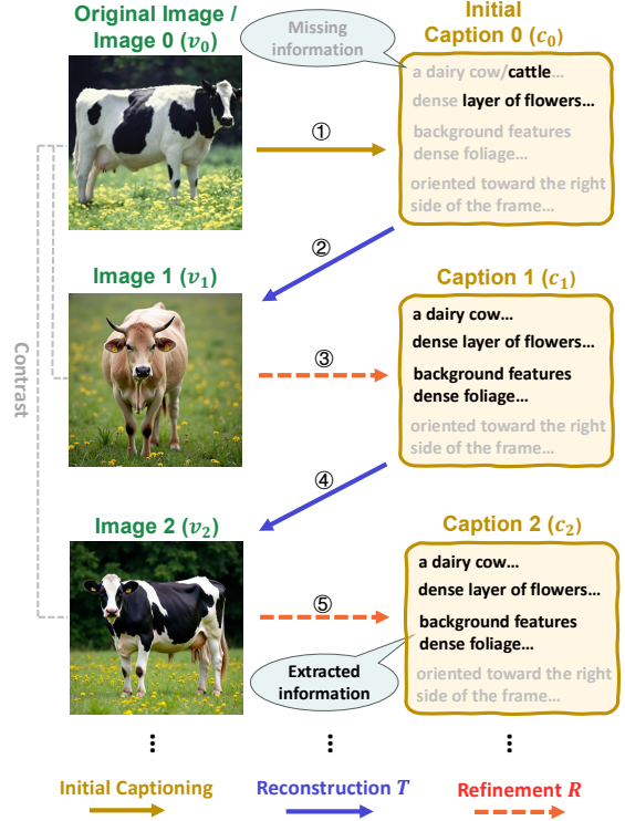
Figure 3: Illustration of the iterative process of RICO. After the initial captioning step, a reconstruction procedure is applied to generate an image from the candidate caption. The caption is then refined by comparing the original image with the reconstructed image.
