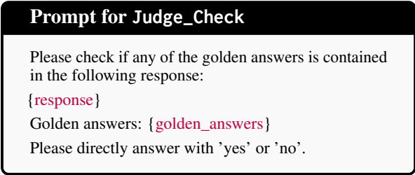
Figure 13: The prompt used for judge_check. Qwen2.5-14B-Instruct-GPTQ-Int4 is used in training, and Claude-3-Haiku is used in evaluation.
