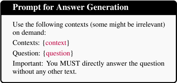
Figure 12: The prompt used for answer generation by frozen LLM.
