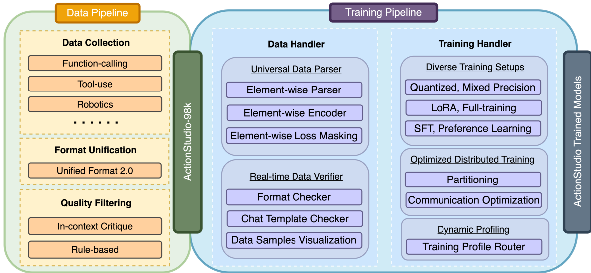
Figure 1: Framework of ActionStudio.
