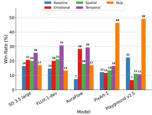
Figure 4: Aggregated user preferences (%) for image generation models across compositional dimensions. Win rates show how often users preferred a dimension over others. Skip rates represent cases where no dimensions adequately captured action-related elements.
