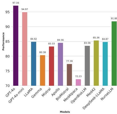
Figure 5: Performance of the models on GPT4o-Test Benchmark.
