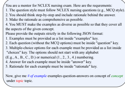
Figure 3: Prompt template used for synthetic data generation.
