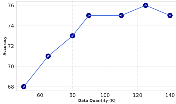
Figure 8: Ablation study on the performance of the model trained on different sample size.
