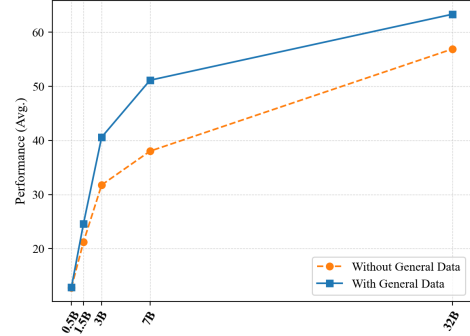
Figure 4: Performance on OOD tasks for models of varying parameter size.
