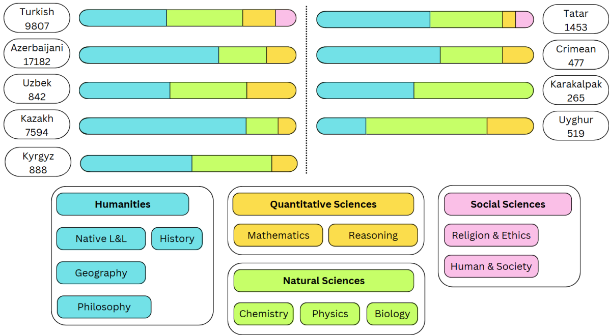
Figure 1. Distribution of subjects across languages in TUMLU. Numbers next to language names indicate the total question count. Left: middle- and high-resource languages; Right: low-resource languages.
