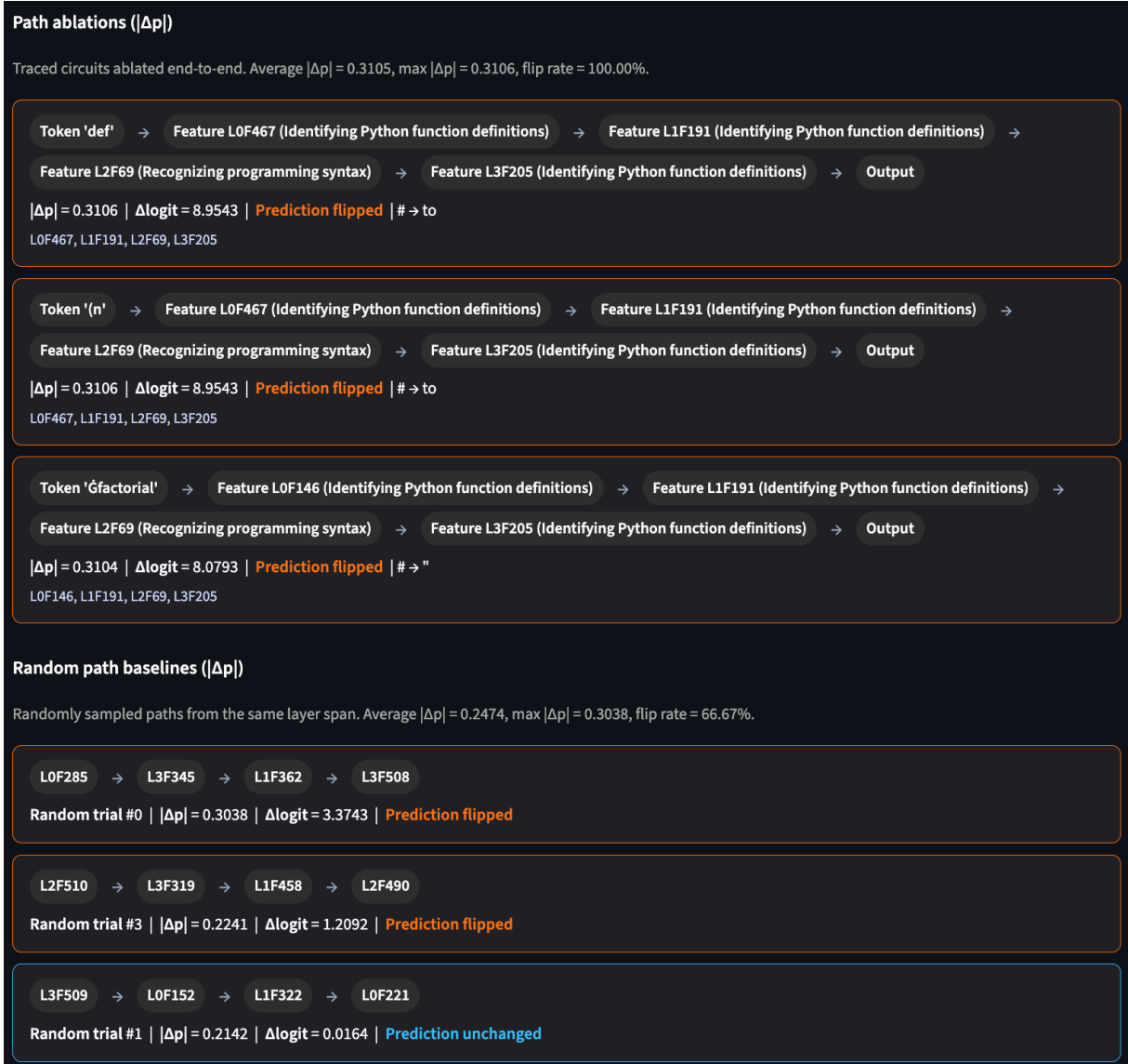
Figure 10: Circuit Trace Analysis: Local path ablations. This view shows the effect of ablating specific paths within the top feature graph shown in the main circuit trace visualization.
