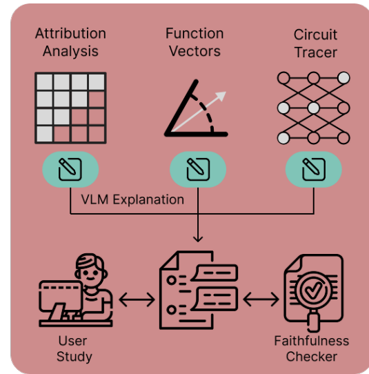
Figure 1: ELIA system overview, including three analysis methods (Attribution Analysis, Function Vectors, and Circuit Tracer) and the explanation generation workflow using VLMs to transform complex interpretability analyses into accessible NLEs. The system is evaluated using a Faithfulness Checker and a user study.
