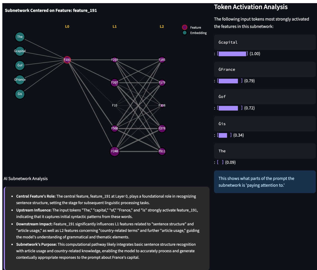
Figure 12: Circuit Trace Analysis: Subnetwork Explorer. This interactive tool allows users to isolate and visualize the specific computational pathways connected to a chosen feature, revealing its upstream influences and downstream effects.
