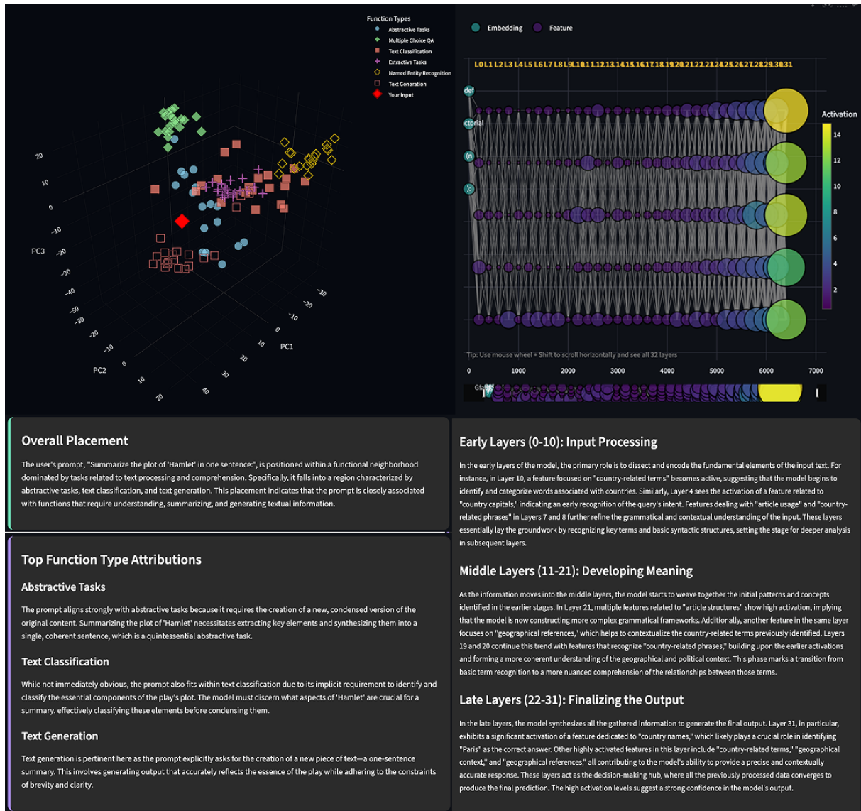
Figure 3: Function Vector and Circuit Trace Analysis visualizations. The 3D PCA plot (left) places the user’s prompt in a semantic functional space, while the Circuit Graph (right) traces the flow of information through interpretable features across layers. Both are accompanied by AI-generated explanations.
