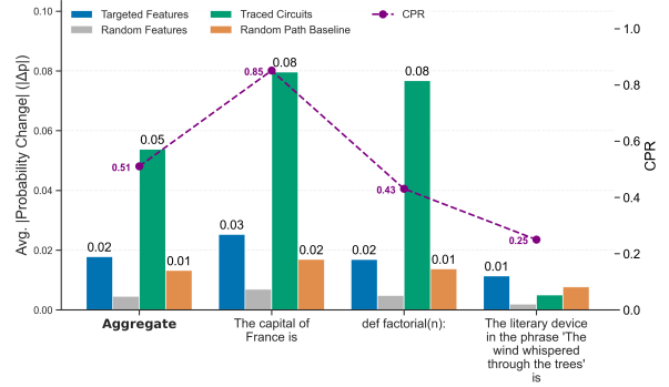
Figure 4: Impact of intervention on model output probability ( |\Delta p| ). We compare the effect of ablating top- k targeted features and traced circuits against random baselines (ablating random features or edges).
