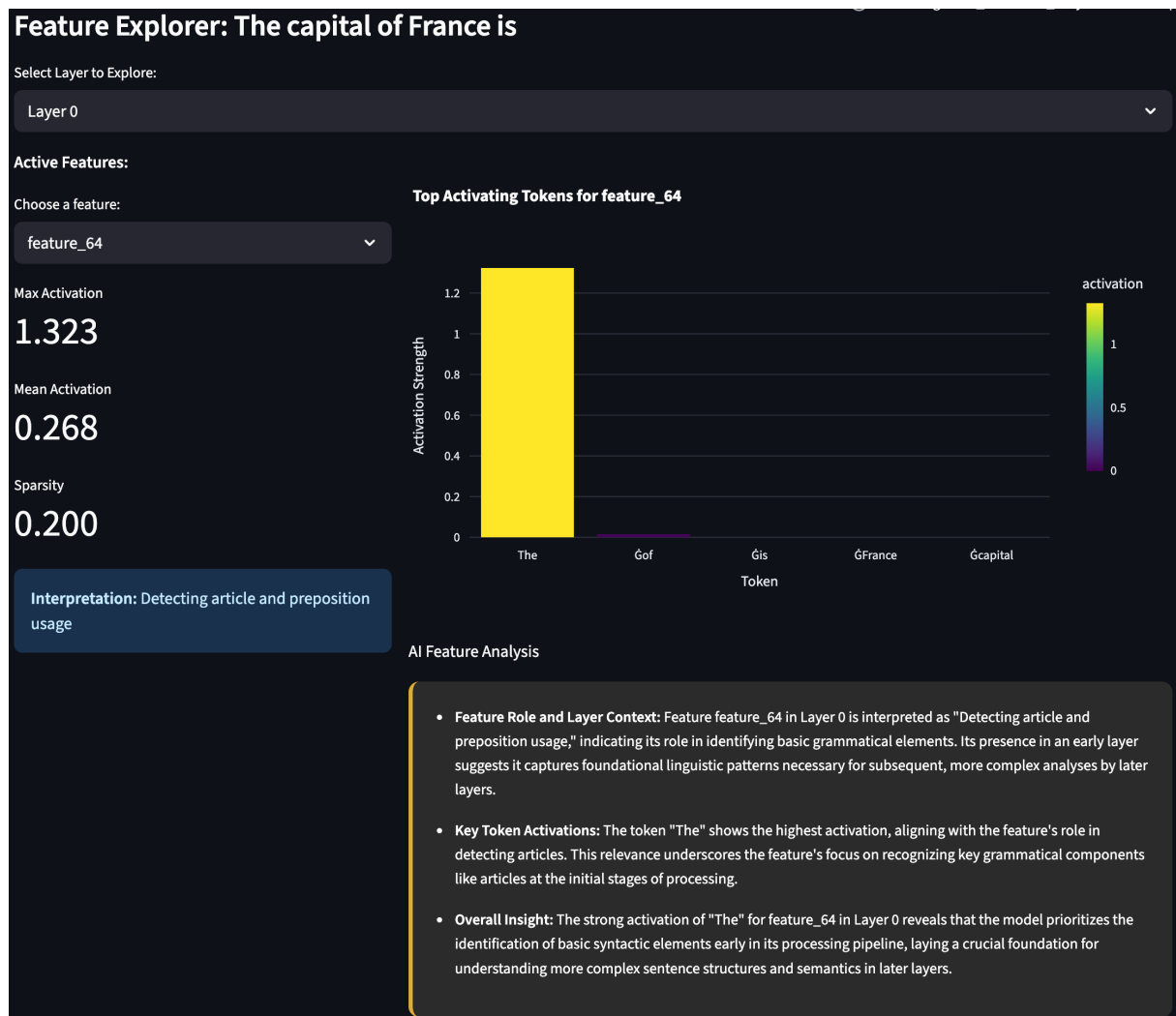
Figure 13: Circuit Trace Analysis: Feature Explorer. Users can inspect individual features in detail, viewing their top activating tokens, sparsity statistics, and AI-generated functional interpretations.
