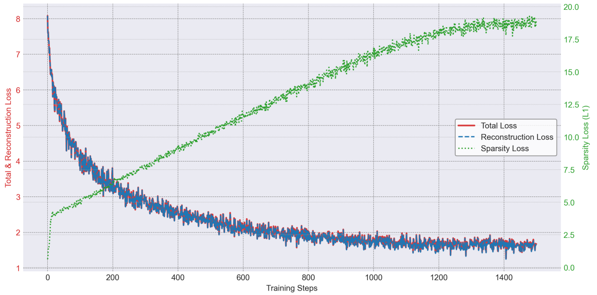
Figure 9: Cross-Layer Transcoder training dynamics showing Total Loss, Reconstruction Loss, and Sparsity Loss ( L_1 ) over 1500 training steps. The CLT is trained on the Dolma dataset with L_1 sparsity regularization, gradient clipping, and cosine annealing learning rate scheduling.
