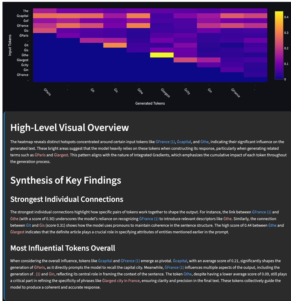
Figure 2: The interactive Attribution Heatmap using Integrated Gradients with an AI-generated natural language explanation. The heatmap visualizes the influence of input tokens on the generated output, and the explanation interprets these results in an accessible narrative.
