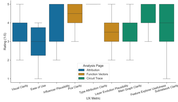
Figure 5: Grouped boxplots of UX ratings for all participants across the three analysis pages.
