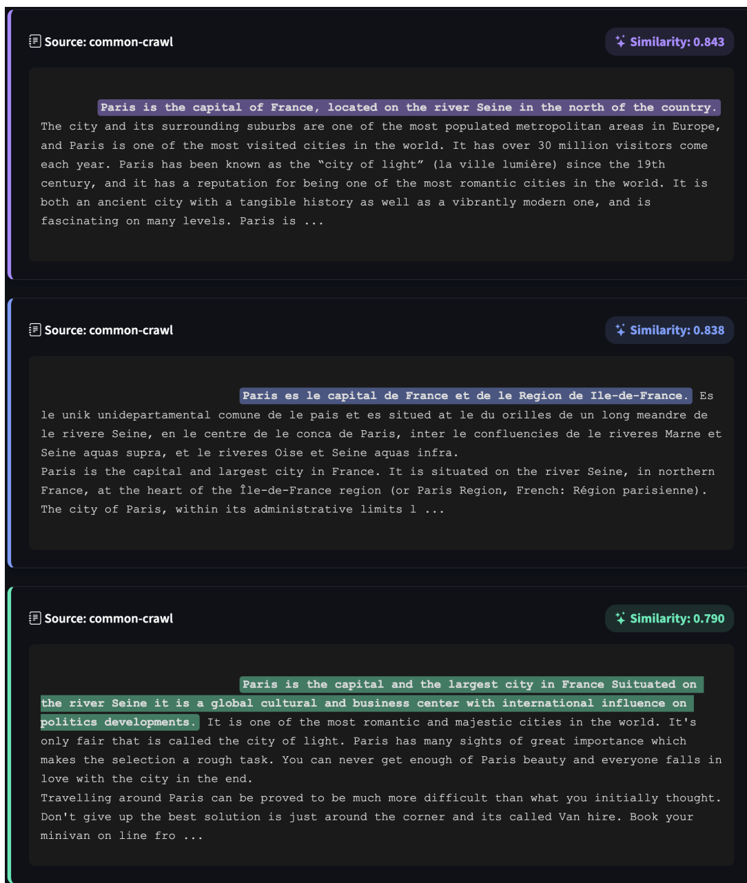
Figure 7: Influence Tracer: Retrieves and displays training documents similar to the prompt.
