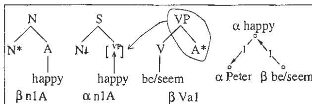
Fig. 4. Derivation tree for Peter is/seems happy
