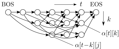
Figure 3: Semi-Markov model representation of NPYLM (simplest case of segment length \leq 3 ). Each node corresponds to a substring ending at time t , and its length k is indexed by each row.
