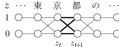
Figure 7: Four types of label transitions in Markov CRF.
