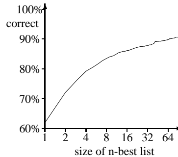
Figure 3: Acceptable NP/PP translations in n-best list for different sizes n
