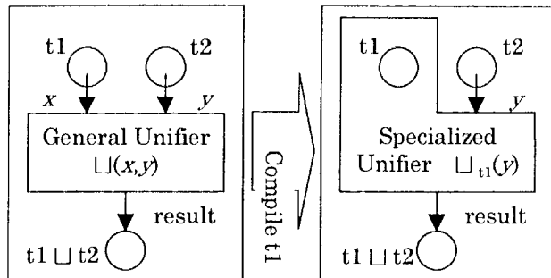
Figure 1 Compiling TFS
