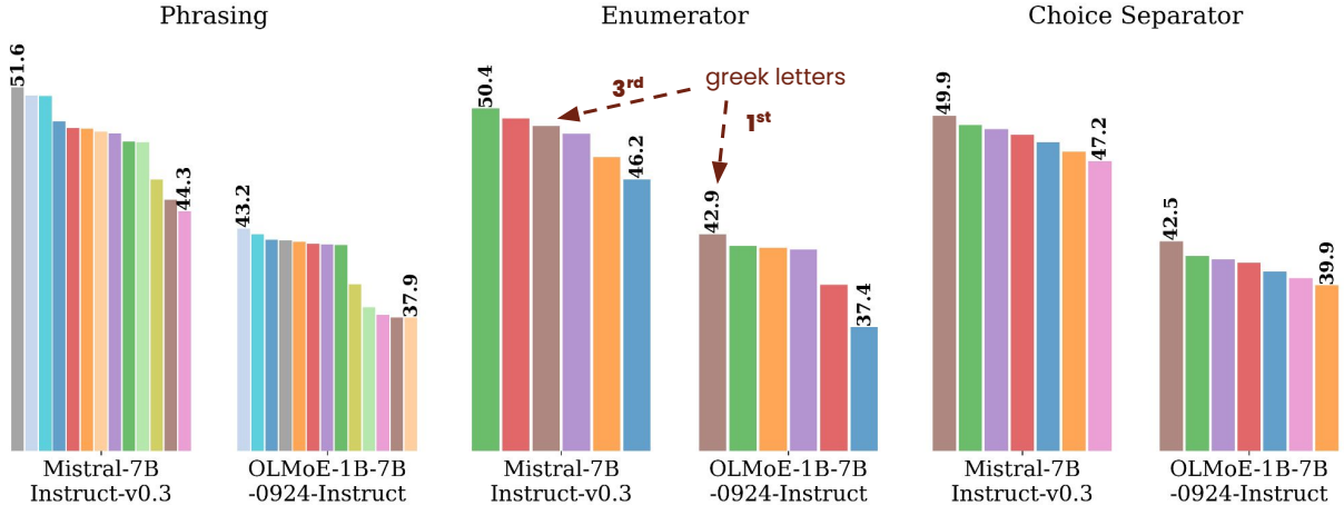
Figure 4: Accuracy marginalization for different dimensions. Variations along each of the dimensions in DOVE lead to prompt sensitivity, even when controlling for all other dimensions.
