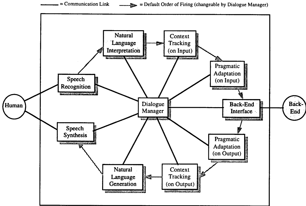
Figure 1. An Architecture for Spoken Dialogue Systems, with Discourse Components in White
