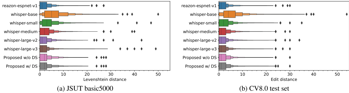
Figure 4: Letter-value plot of Levenshtein distance for the comparison of the proposed model with the publicly available ASR models. The proposed model employed greedy search, while the comparative models used beam search with a beam size of 5. “DS” denotes DeepSpeed-Inference.
