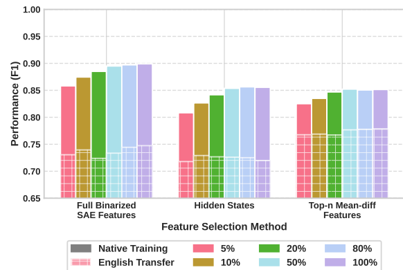
Figure 1: Multilingual performance comparison across three feature selection methods under varying training data sampling rates. Solid bars represent models trained on native language data, while hatched bars show performance with English transfer learning. Binarized SAE features demonstrate robustness across different training data constraints.
