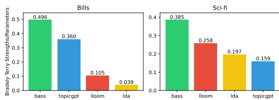
Figure 3: BASS has the highest preference strengths than other groups on both datasets, where users using BASS generate better responses than unsupervised topic models. However, the position of TopicGPT swaps from Bills to Sci-Fi, where TopicGPT only generates one super topic and three subtopics for Sci-Fi (§ 6.1).
