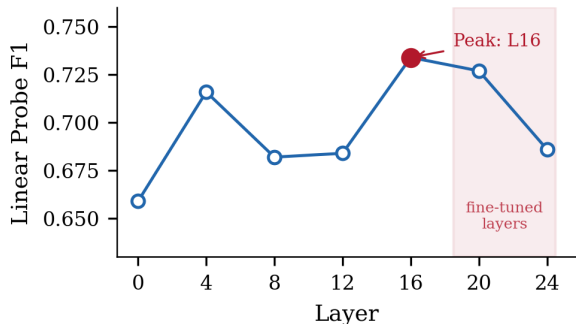
Figure 2: Linear probe F1 by encoder layer. Inverted-U curve peaks at layer 16/24. Shaded region: fine-tuned layers (19–24).
