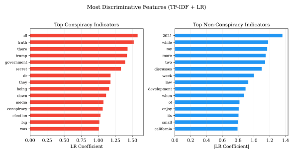
Figure 5: Top discriminative TF-IDF features by class. Believers favor third-person agentive referents and certainty markers; non-believers use first-person epistemic hedges and meta-cognitive verbs.
