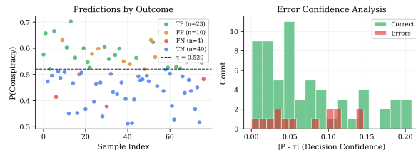
Figure 4: Prediction confidence by outcome. 13 of 14 errors fall in the low-confidence zone ( 0.4 < p < 0.6 ); false positives dominate, consistent with narrative density.
