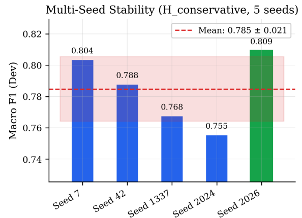
Figure 7: Per-seed F1 variation. Single-seed results are unreliable ( \sigma = 0.021 ); probability averaging over 5 seeds corrects boundary disagreements.
