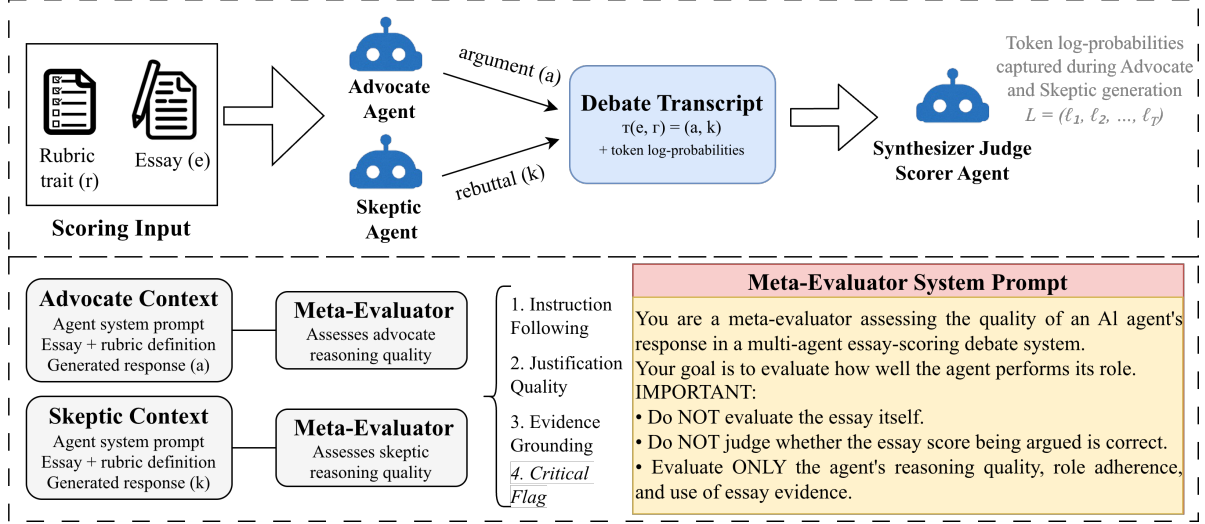
Figure 1: Overview of the proposed multi-agent debate and LLM-as-judge evaluation framework.
