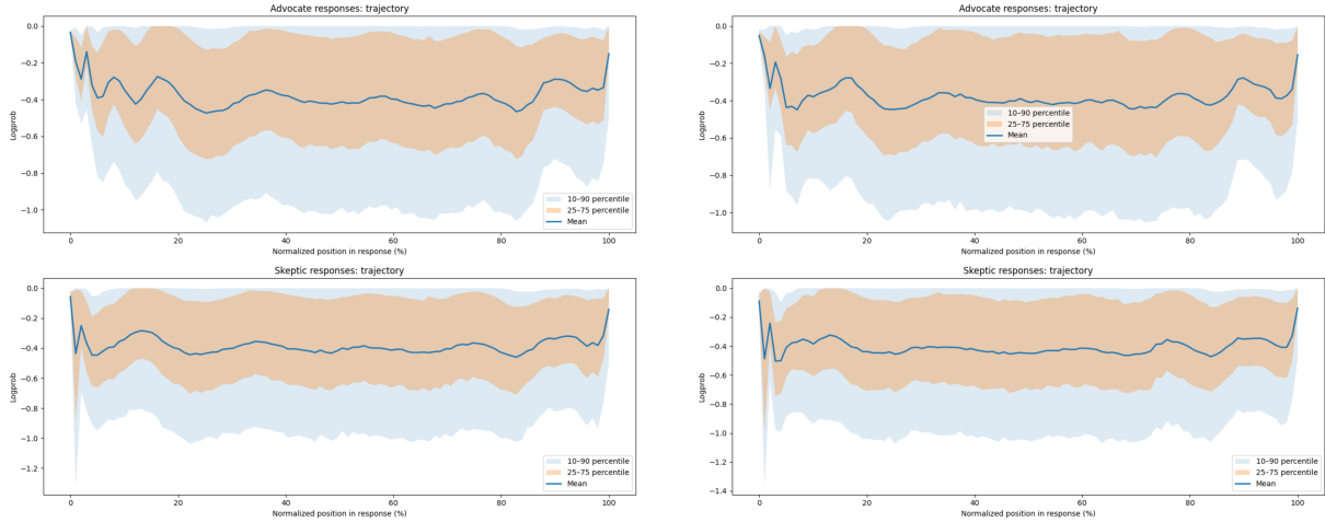
Figure 2: Token-level log-probability trajectories for Advocate and Skeptic responses on Essay Sets 7 (left) and 8 (right). Solid lines denote mean trajectories; shaded regions indicate percentile bands (25–75 and 10–90).
