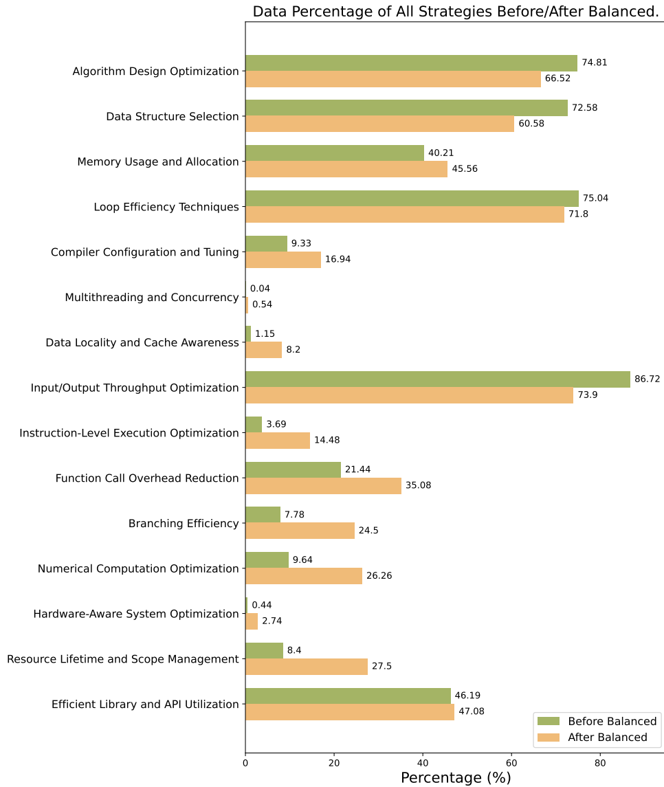
Figure 5: An illustration of data percentage of strategies in the training data before or after balanced sampling.
