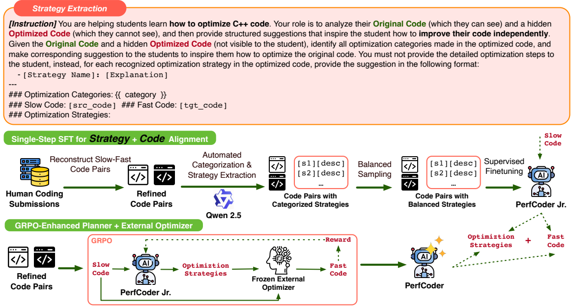
Figure 2: An illustration of our PerfCoder framework.
