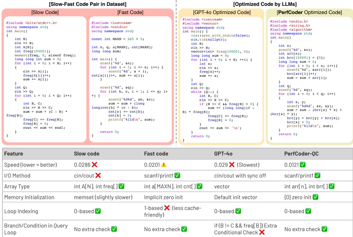
Figure 1: A real code optimization case of PerfCoder and ChatGPT.
