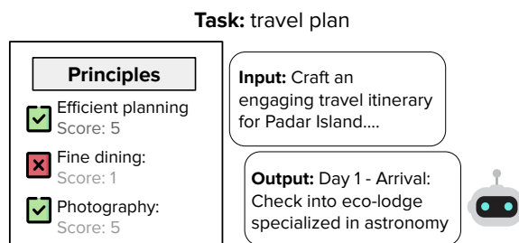
Figure 1: Humans often rely on implicit principles when assessing an LLM’s output for a given task. For instance, when asking an LLM to design a travel itinerary, they may judge the output favorably if it reflects their principle of efficient planning and meets their preferred requirements such as including good photography locations. We extend this evaluation phase to large-scale automated data generation by leveraging LLMs to generate a broader variety of such principles.
