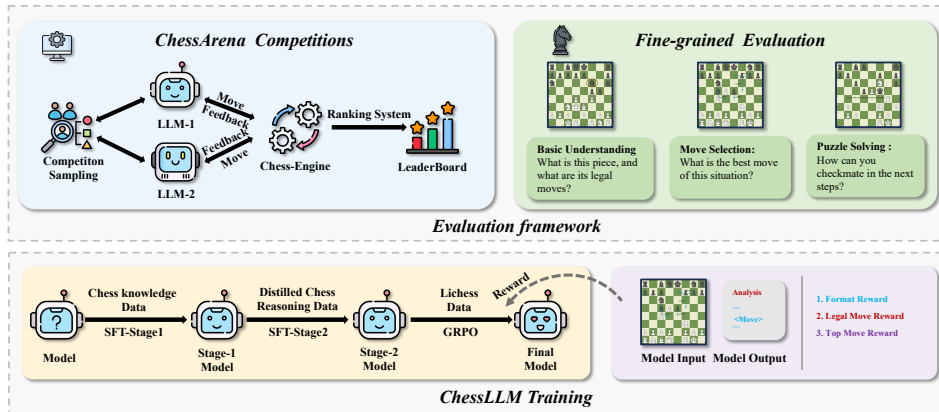
Figure 1: Overview of ChessArena competitions, fine-grained evaluation, and ChessLLM training. (1) An LLM can be integrated into ChessArena to compete against other models. After a certain number of competitions, each model is assigned a reliable Glicko rating and added to the leaderboard. (2) Three additional evaluation tasks are integrated into ChessArena to evaluate the chess capabilities at a fine-grained level. (3) We can extract high-quality chess reasoning data from the gameplay process, which can be used for training an LLM specially for chess.
