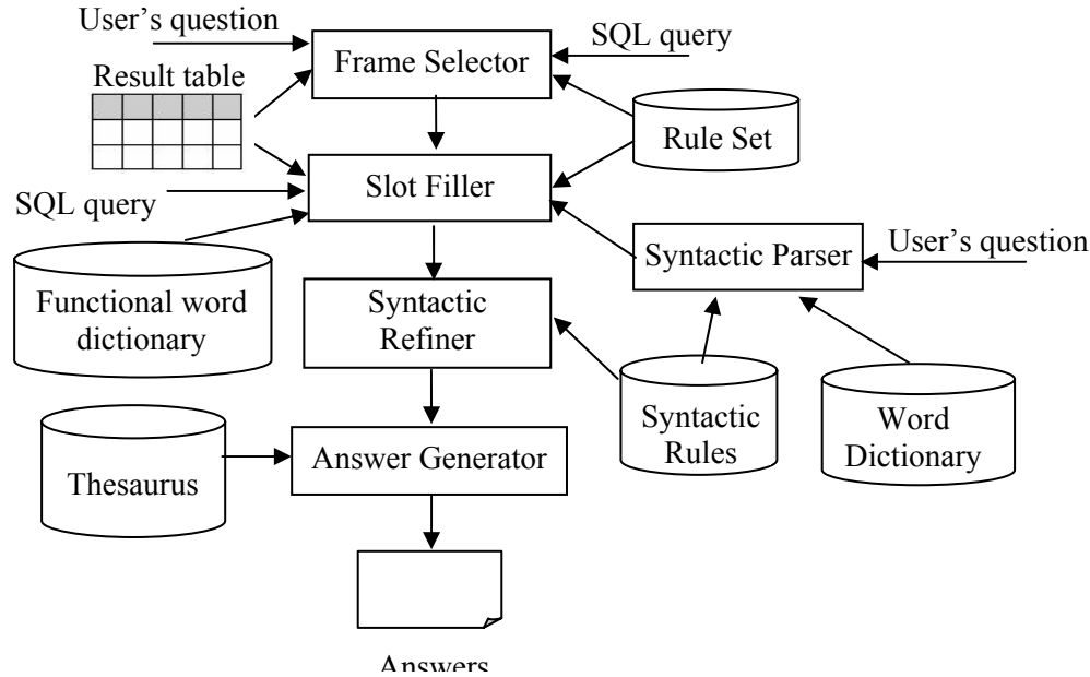
Figure 3: Data flow in the Text Generator
