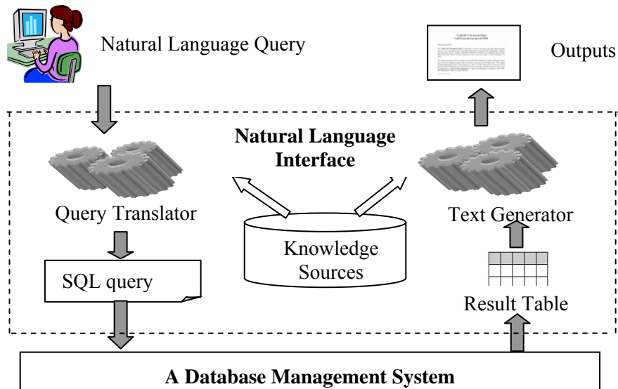
Figure 1: Architecture of the NLI4DB
